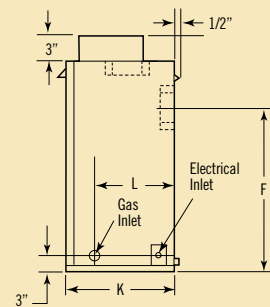
Right Side View (Rear vent shown)
